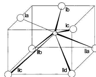
Figure 2. Monoclinic ZrO 2 . Small circle = zirconium atom; large circles = oxygen atoms.
